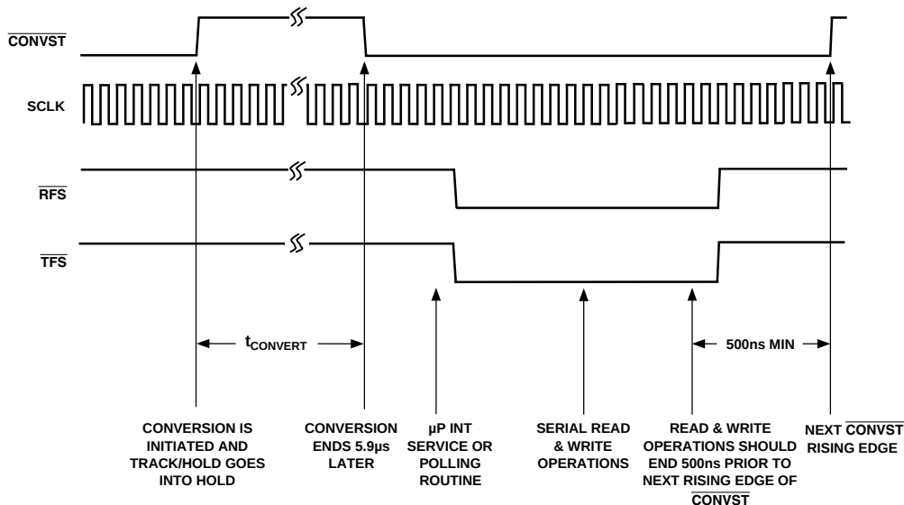
Figure 4. Sequence Using CONVST as an Interrupt Signal
