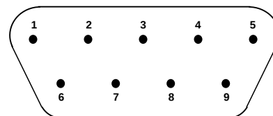
Figure 2. Pin Configuration for SKT14, D-Type Connector
